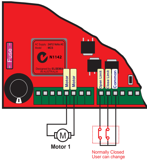
Controller with limits connected
