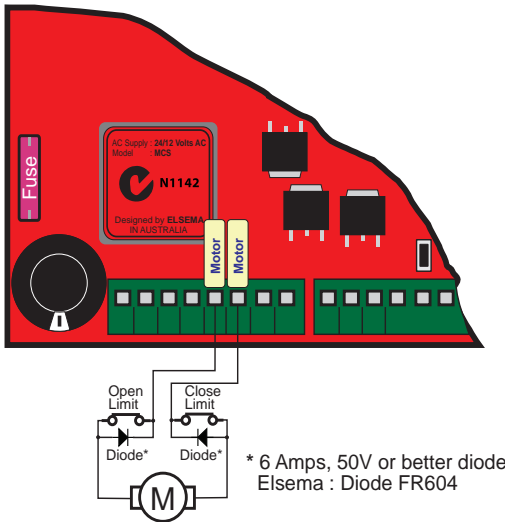
Controller with limits in series with motor
